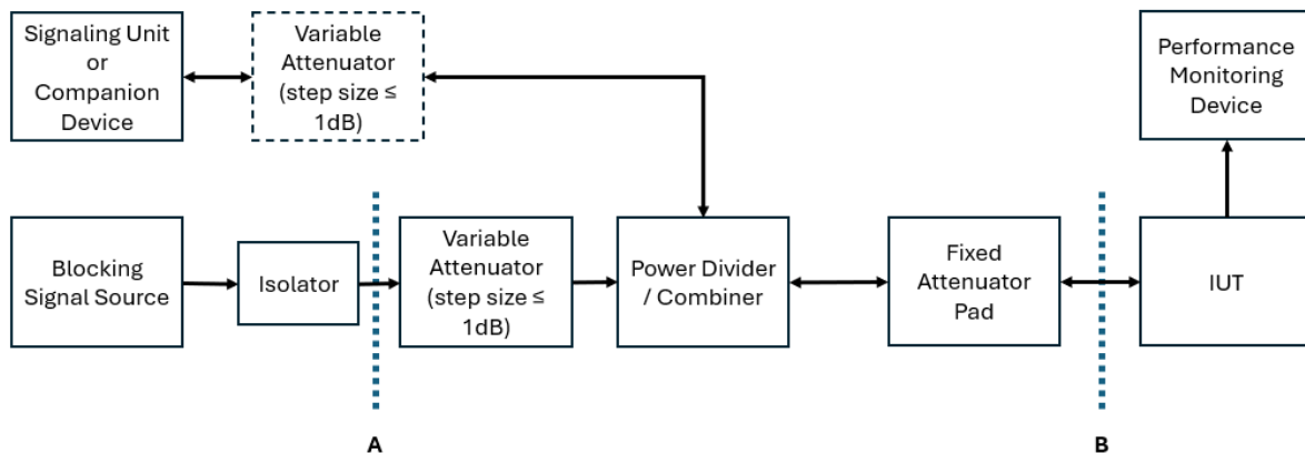
Figure 3.1: Test setup for receiver blocking
